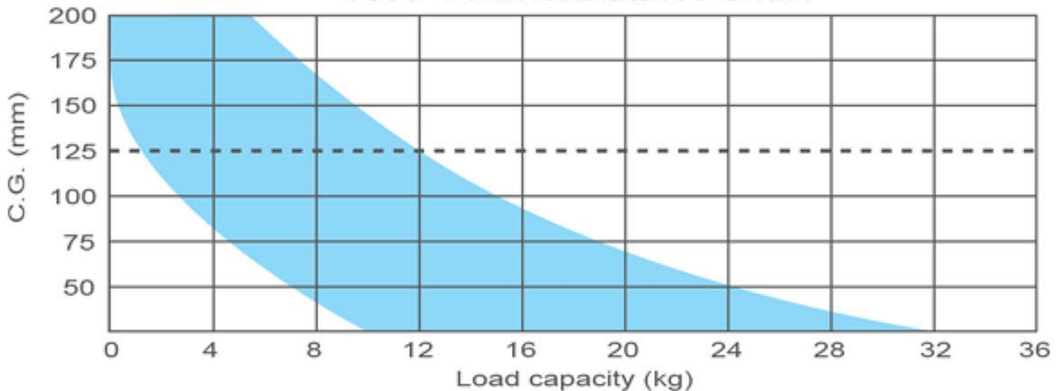
CH6 Counterbalance chart
